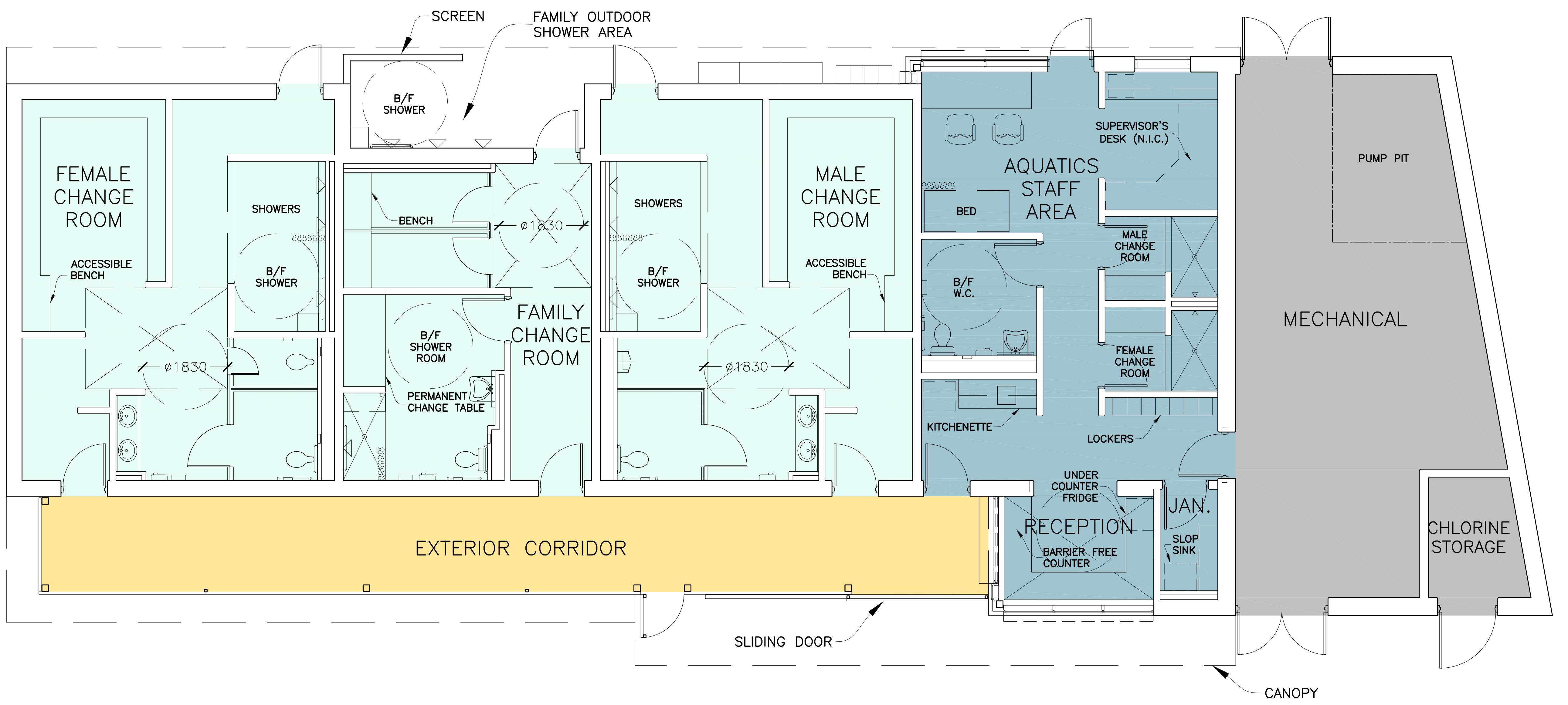
PLAN
